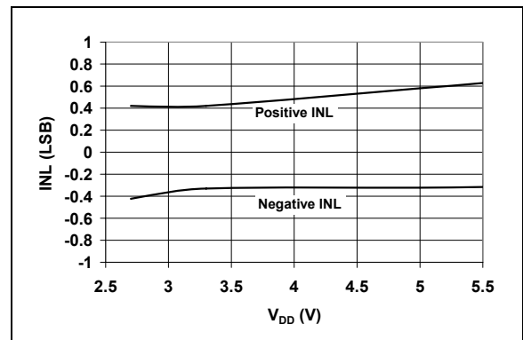
FIGURE 2-5: INL vs. V_{DD} - I^2C^{\text{TM}} Fast Mode ( f_{SCL} = 400\text{ kHz} ).
