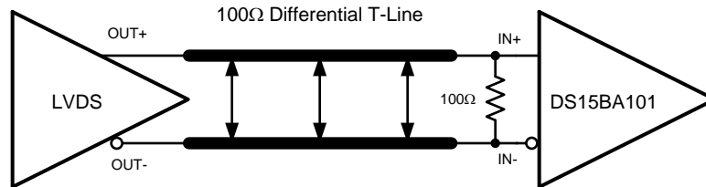
Figure 3. Typical LVDS Driver DC-Coupled Interface to DS15BA101 Input
