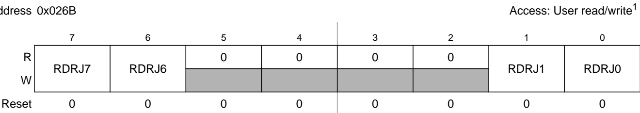
Figure 2-59. Port J Reduced Drive Register (RDRJ)
