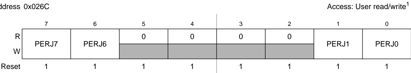
Figure 2-60. Port J Pull Device Enable Register (PERJ)
