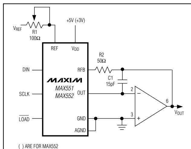
Figure 3. Unipolar Operation
