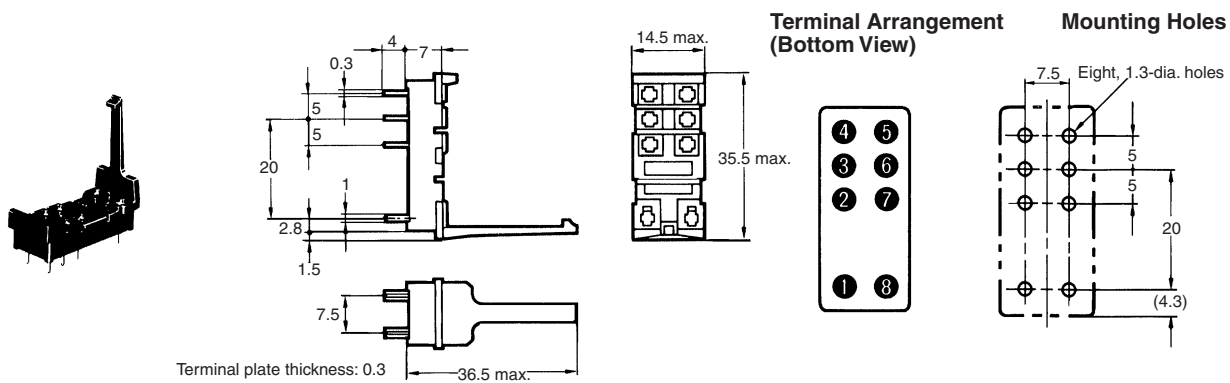
P2R-08P (2-pole)
