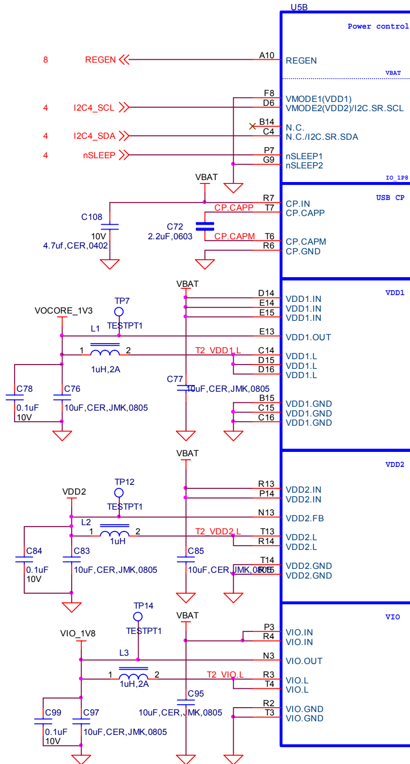
Figure 24. Main Power Rails
