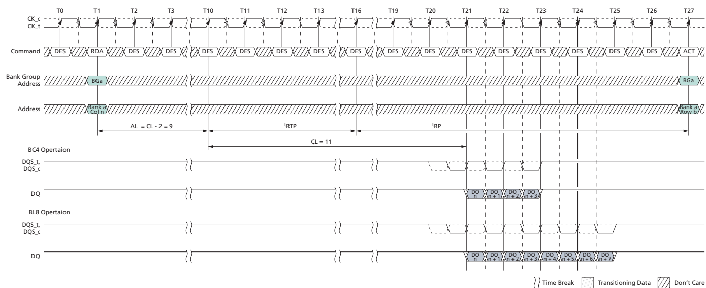
Figure 152: READ with Auto Precharge, Additive Latency, and 1 st CK Preamble
