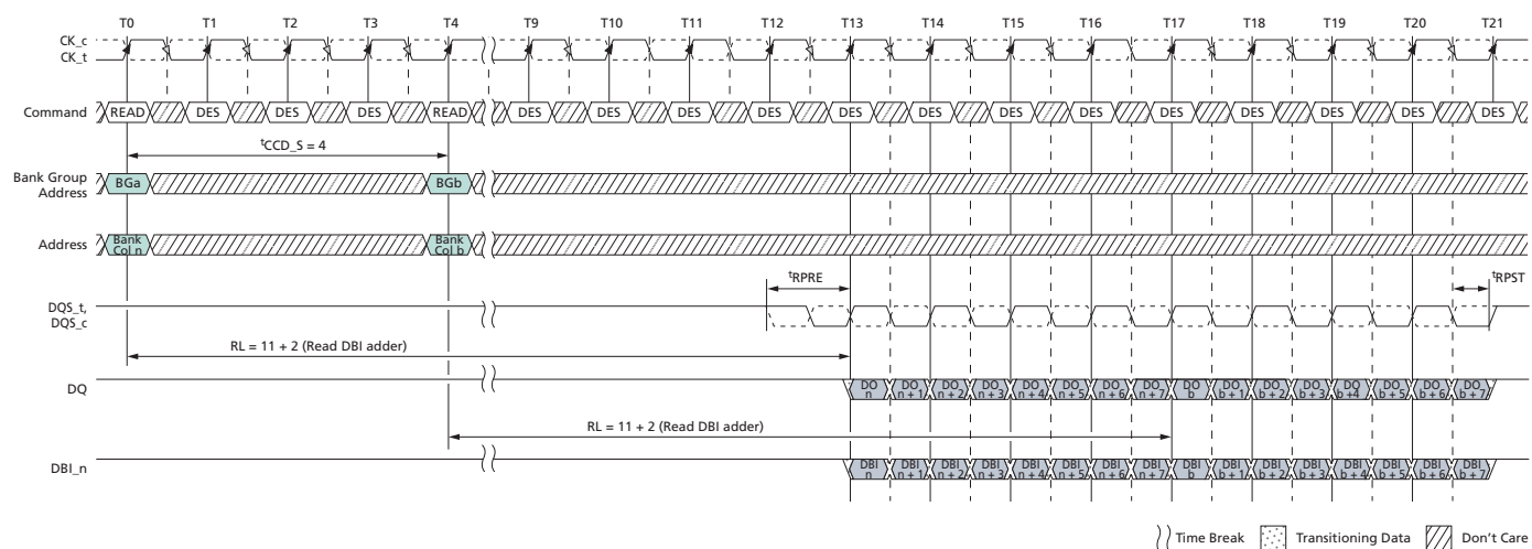
Figure 153: Consecutive READ (BL8) with 1 st CK Preamble and DBI in Different Bank Group
