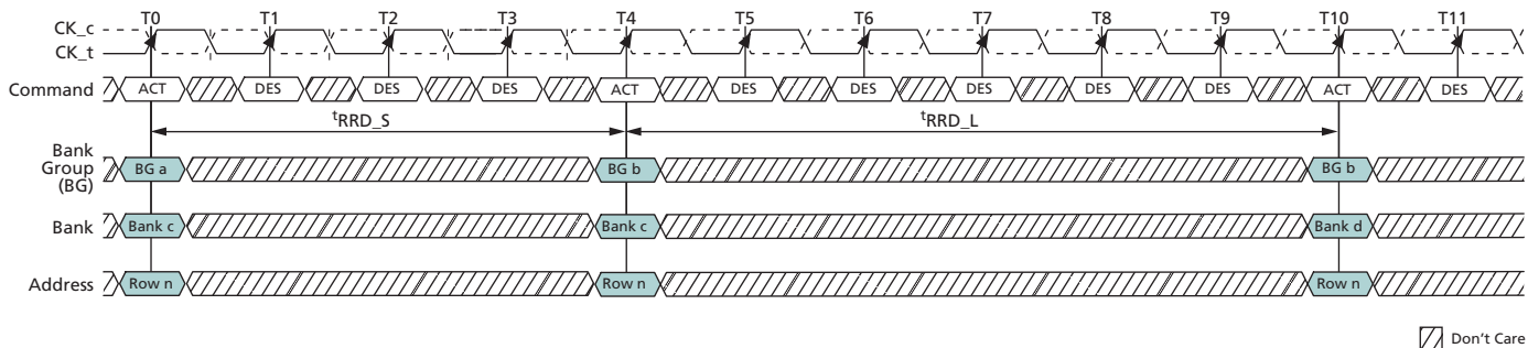
Figure 117: t_{RRD} Timing
