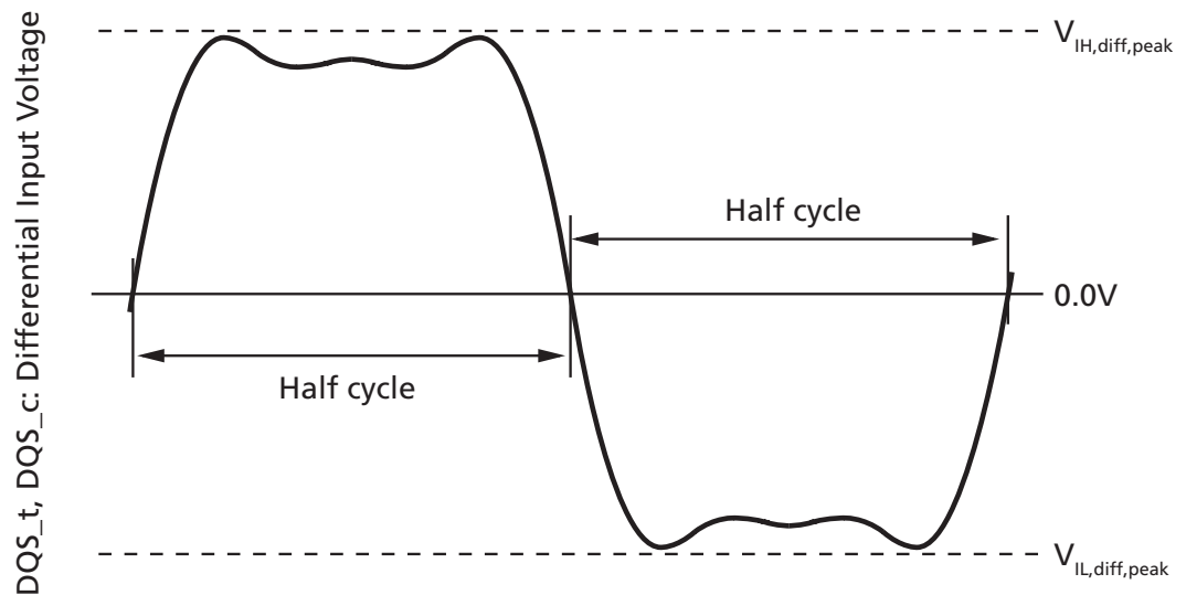
Figure 220: Differential Input Signal Definition for DQS t , DQS c
