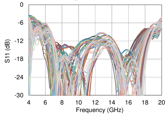
Input Return Loss vs. Frequency All phase states, 25C
