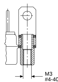
Plastic Bracket with Post (1APN/1A6N)
