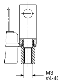
Metal Bracket with Post (1AHN/1A8N)
