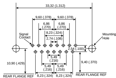
15 Contacts
