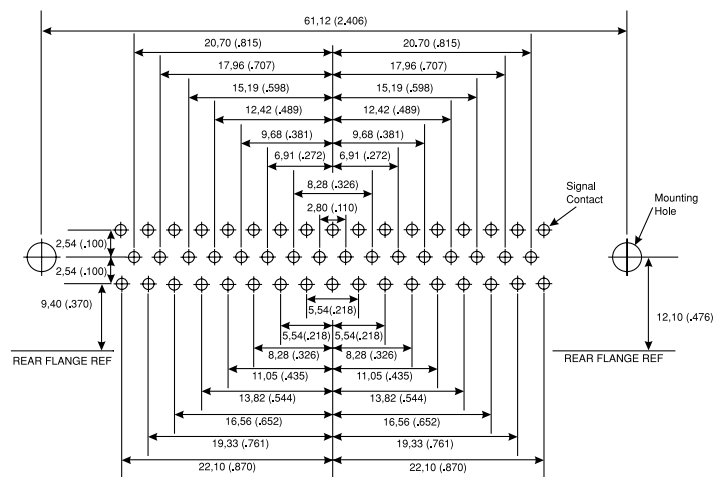
50 Contacts
