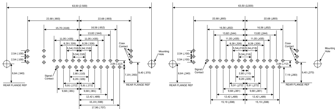
Shell Size Contact Arrangement No. of Size 20 Cavities No. of Size 8 Cavities C 25W3 22 #20 3 #8 Shell Size Contact Arrangement No. of Size 20 Cavities No. of Size 8 Cavities C 27W2 25 #20 2 #8
