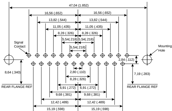
25 Contacts
