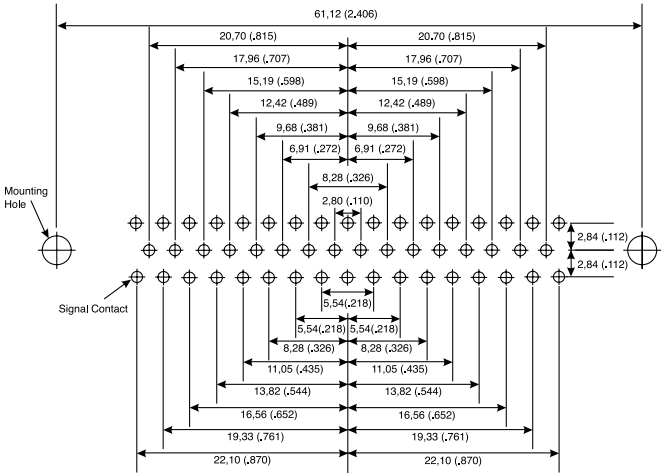
50 Contacts
