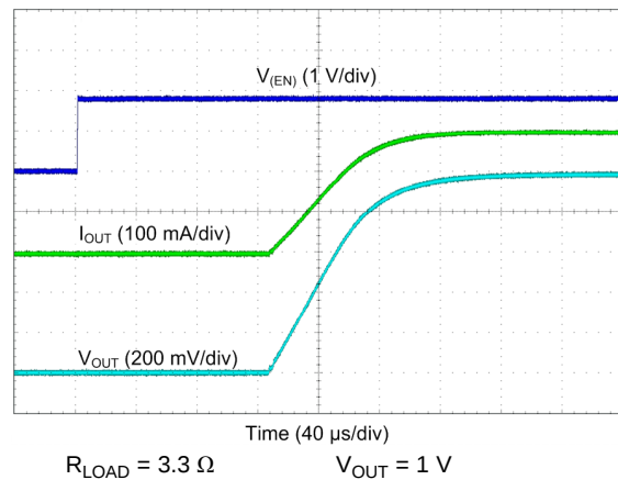
Figure 74. LDO Start-Up
