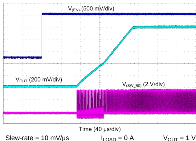
Figure 46. Buck Start-Up With EN1, Forced PWM Mode (Single-Phase Output)
