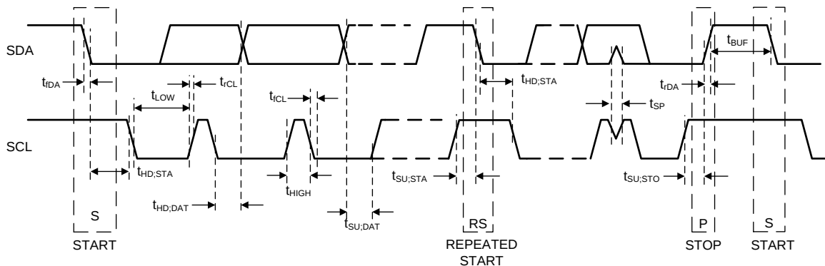
Figure 25. I²C-Compatible Timing
