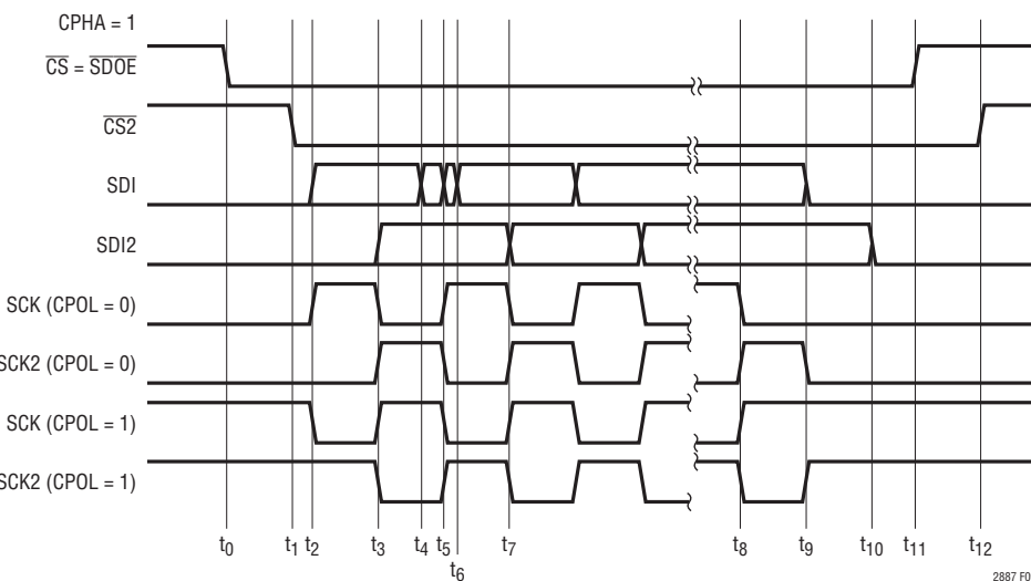
Figure 9. SPI Timing, Unidirectional, CPHA = 1
