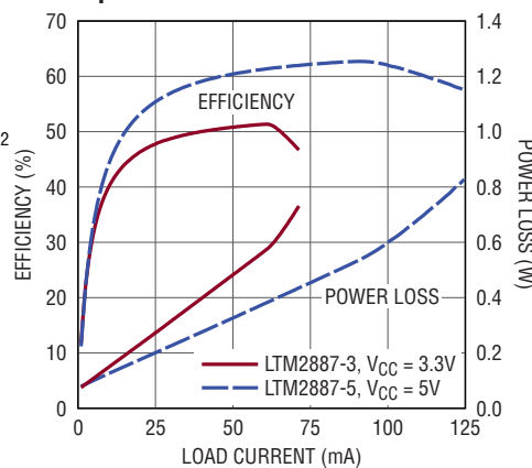
V_{CC2} and V_{L2} Efficiency with Equal Load Current
