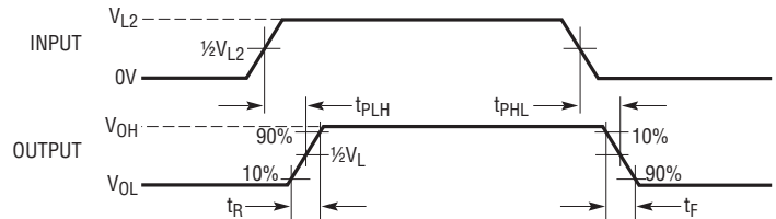
Figure 1. Logic Timing Measurements
