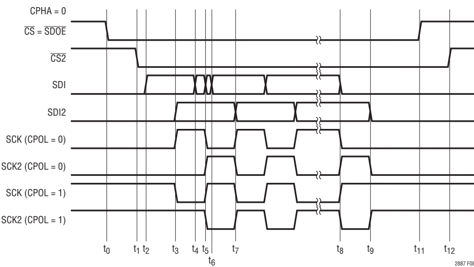
Figure 8. SPI Timing, Unidirectional, CPHA = 0
