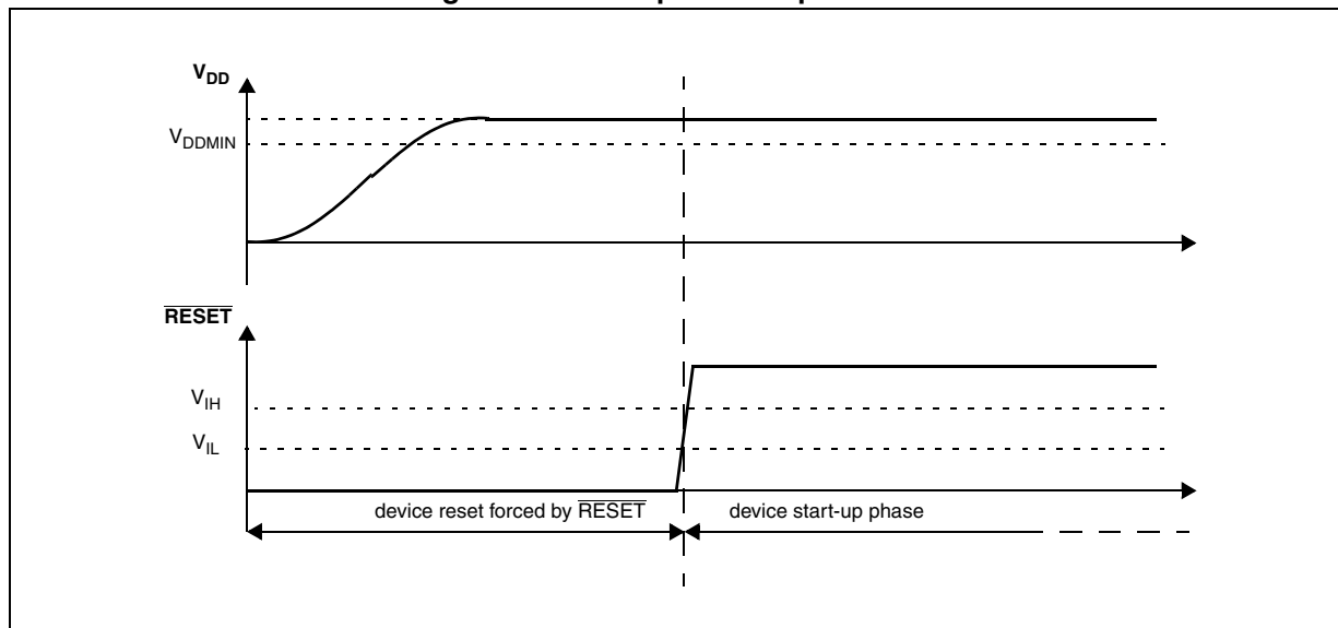
Figure 16. Start-up reset requirements
