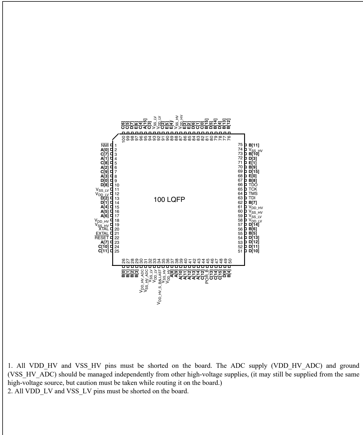
Figure 3. 100-pin LQFP pinout (top view) 1
