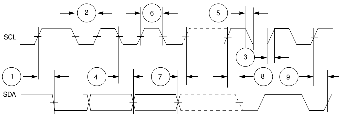
Figure 35. I²C input/output timing
