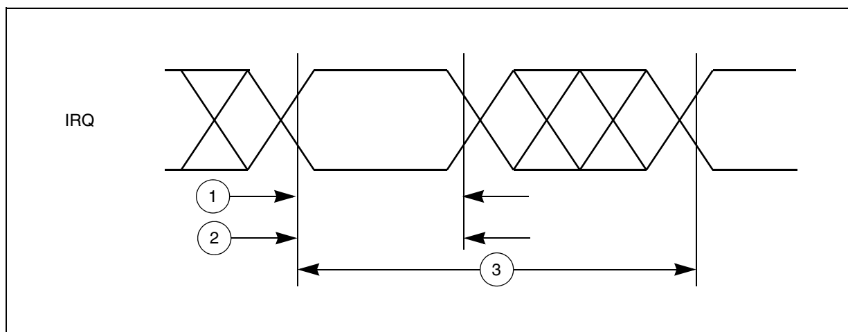
Figure 21. External interrupt timing
