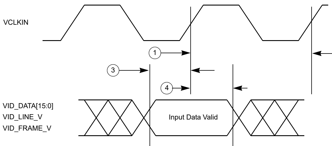
Figure 31. Video interface timing
