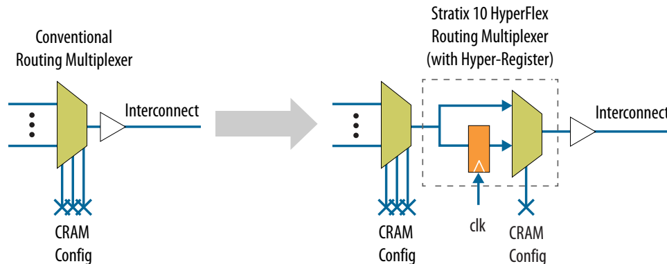
Figure 3. Bypassable Hyper-Register
