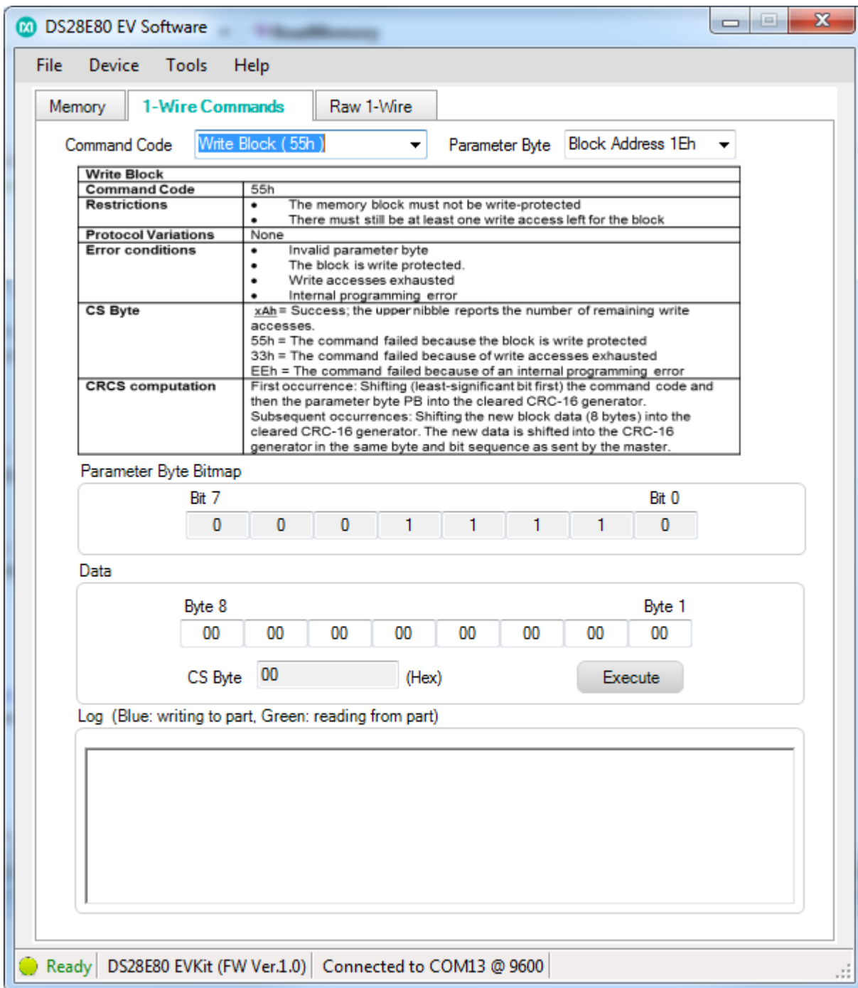
Figure 16. 1-Wire Commands Tab Selected
