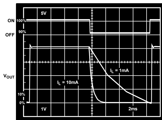
Figure 16. SLEEP Response Time
