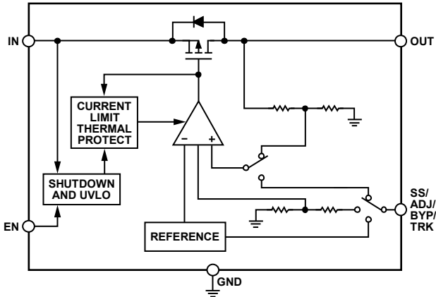
Figure 25. Internal Block Diagram
