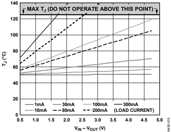
Figure 37. 100 mm 2 of PCB Copper, T A = 50°C
