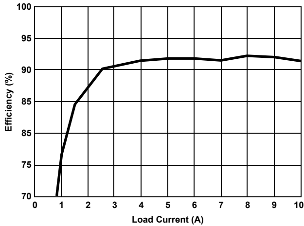
Figure 18. Efficiency vs Load V_{IN} = 48V
