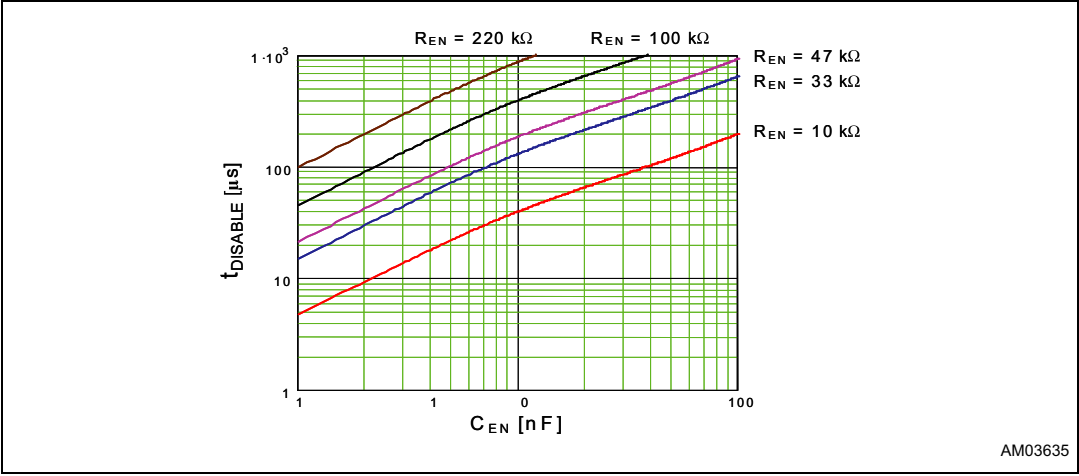
Figure 21. t_{\text{DISABLE}} versus C_{\text{EN}} and R_{\text{EN}}
