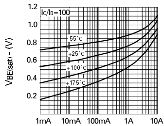
I_C -Collector Current
