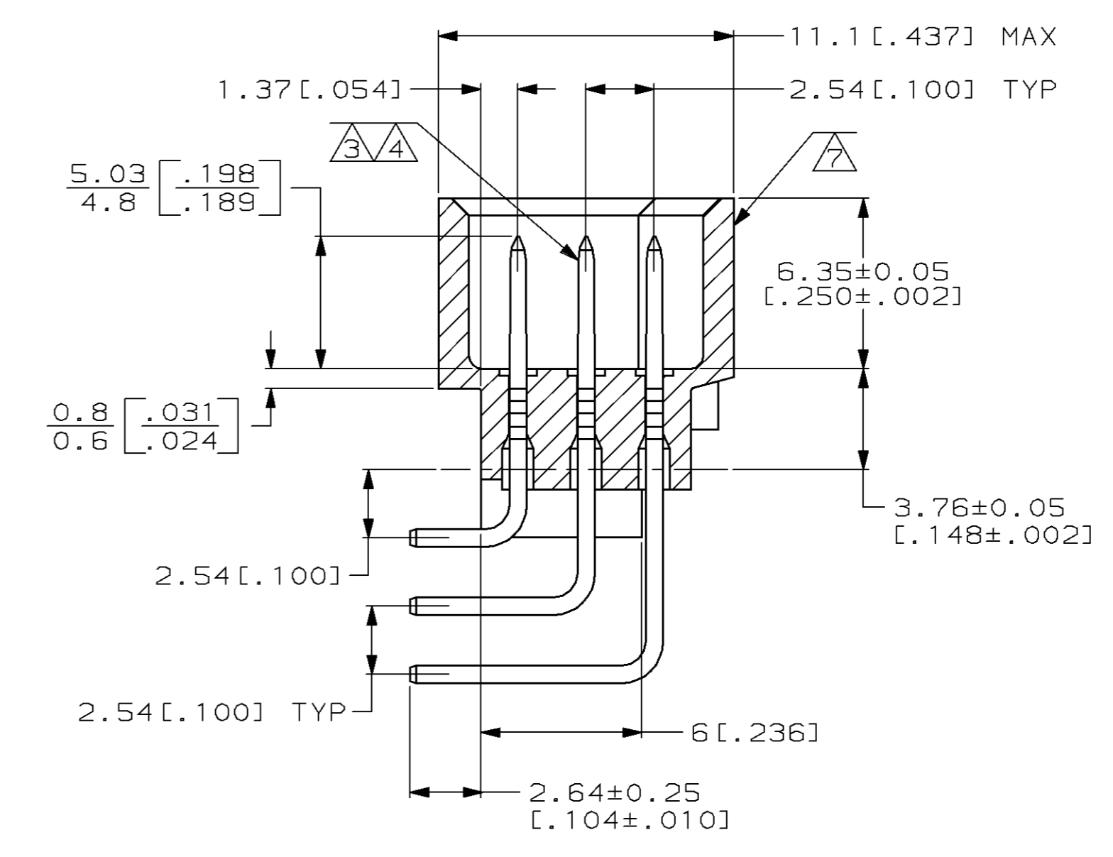
SECTION Z-Z
