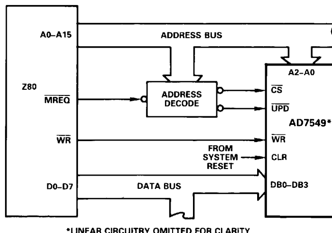
Figure 6. AD7549-Z80 Interface
