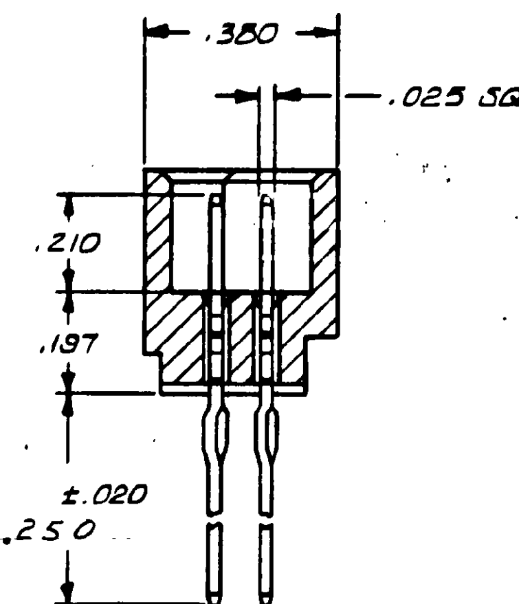
SECTION X-X
