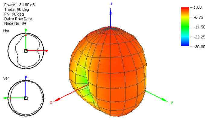
Figure 17. Radiation Pattern at 850 MHz of FXUB70 Port 2.
