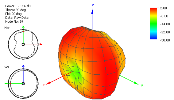
Figure 25. Radiation Pattern at 1850 MHz of FXUB70 Port 2.
