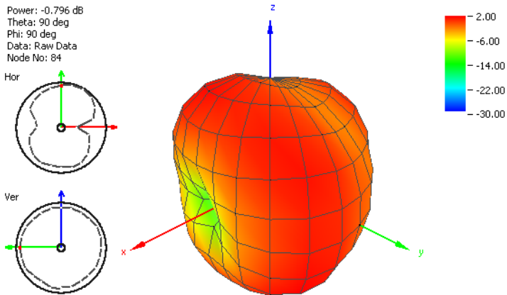
Figure 20. Radiation Pattern at 1575 MHz of FXUB70 Port1
