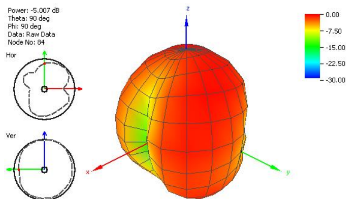
Figure 19. Radiation Pattern at 925 MHz of FXUB70 Port 2.
