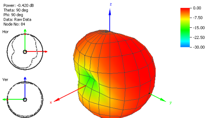
Figure 18. Radiation Pattern at 925 MHz of FXUB70 Port 1.
