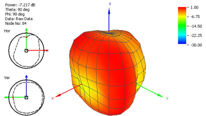
Figure 23. Radiation Pattern at 1750 MHz of FXUB70 Port 2.
