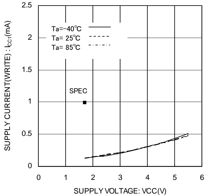
Figure 13. Supply current (WRITE) I_{CC1}(WRITE, f_{SK}=1MHz)
