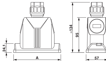
Dimensional drawing with letter dimension A
