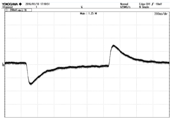
Figure 5: Output voltage response to step-change in load current (50%-75%-50% of full load; di/dt = 0.1A/\mu s ). Trace: Vout; 200mV/div; Time: 200us/div
