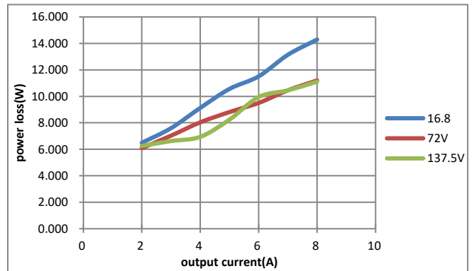
Figure 2: Power loss vs. load current for 16.8, 72V and 137.5V input voltage at 25°C.
