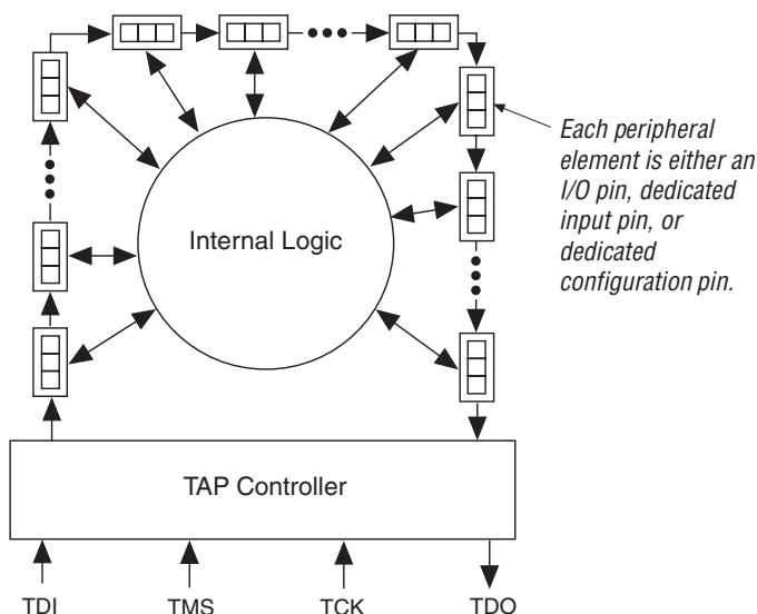
Figure 14–3. Boundary-Scan Register
