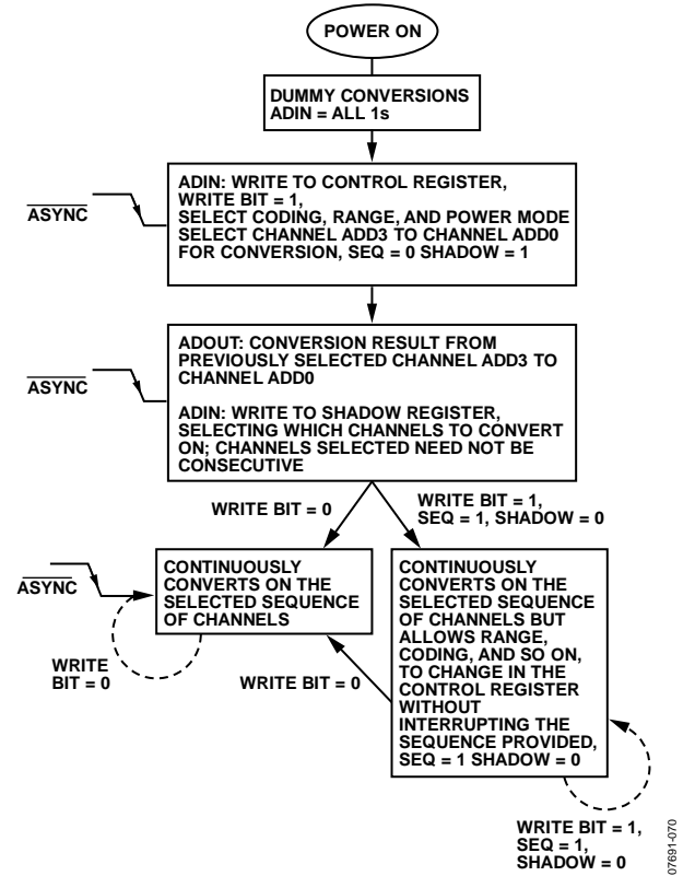
Figure 70. Continuous Conversions
