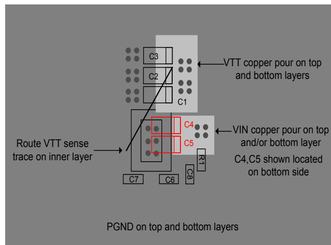
Figure 3 — Component Placement and Layout
