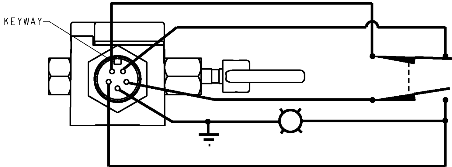
MODIFICATION CODE G WIRING DIAGRAM
