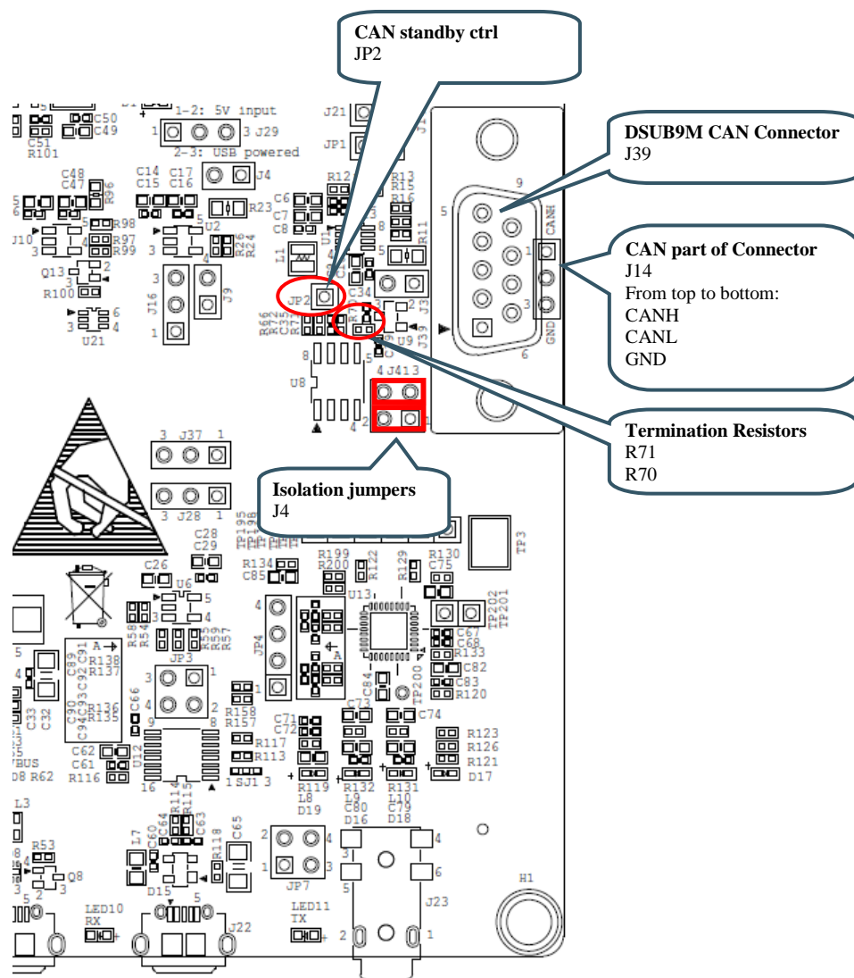
Figure 21 – CAN Interface
