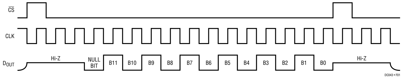
Figure 1. Timing Diagram
