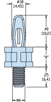
BAYONET SNAP LOCK 10,2 / M4 MALE THREAD
