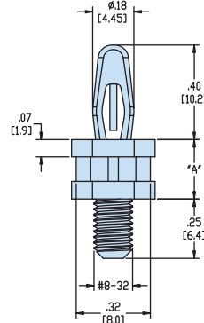
BAYONET SNAP LOCK 10,2 / 8-32 MALE THREAD
