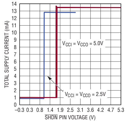
Total Supply Current vs SHDN Pin Voltage
