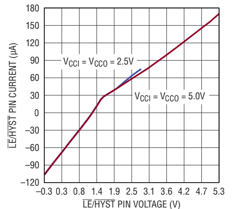
LE/HYST Pin I-V Characteristics
