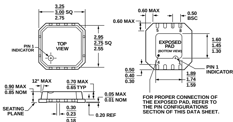
Figure 44. 8-Lead Lead Frame Chip Scale Package [LF CSP_VD] 3 mm x 3 mm Body, Very Thin, Dual Lead (CP-8-2) Dimensions shown in millimeters
