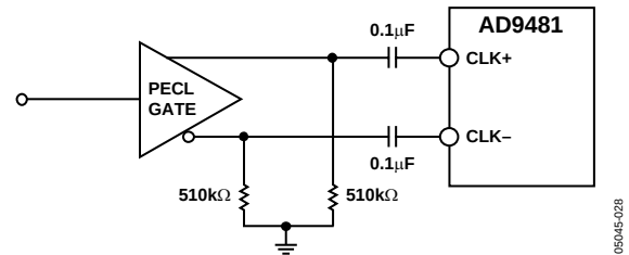
Figure 37. Clocking the AD9481
