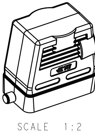
TYPE-6:H0B HOOD,HIGH CONSTRUCTION, NO ENTRY,2 EAR OTHER SPEC REFER TO TYPE-3 类型-6:H10B上壳,高结构,无出线孔,2耳 其它规格尺寸参照类型-3
