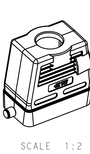
TYPE-4:H10B HOOD,HIGH CONSTRUCTION, TOP ENTRY,2 EAR 类型-4:H10B上壳,高结构,顶出,2耳
