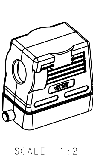
TYPE-3:H10B HOOD,HIGH CONSTRUCTION, SIDE ENTRY,2 EAR 类型-3:H10B上壳,高结构,侧出,2耳
