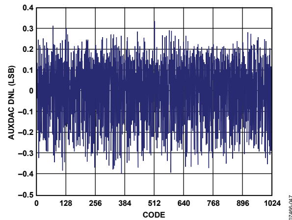
Figure 40. AUXDAC DNL
