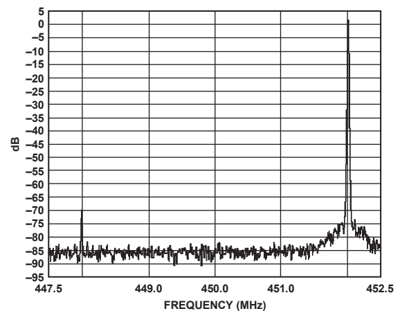
Figure 96. AD9114/AD9115/AD9116/AD9117 and ADL5370 with a Single-Tone Signal at 450 MHz, Gain and LO Compensation Optimized
