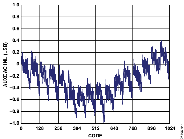
Figure 37. AUXDAC INL
