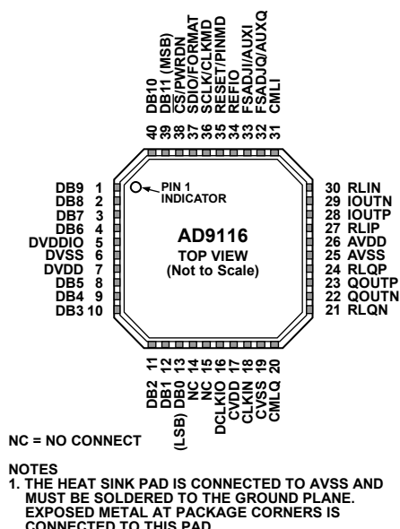
Figure 3. AD9116 Pin Configuration
