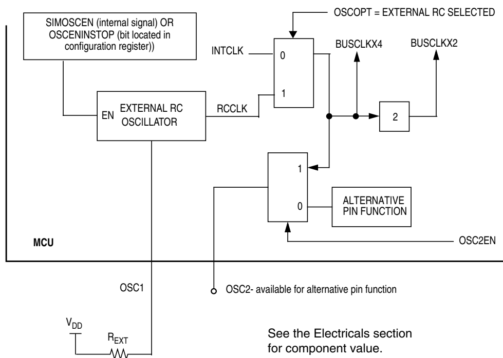
Figure 10-3. RC Oscillator External Connections
