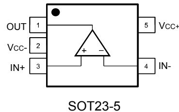
Figure 1. Pin connections (top view)
