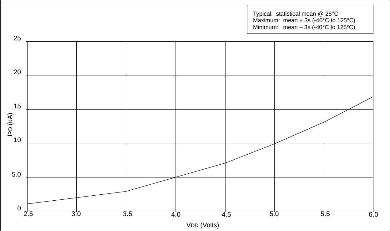
FIGURE 18-6: TYPICAL I PD vs. V DD , WATCHDOG ENABLED (25°C)
