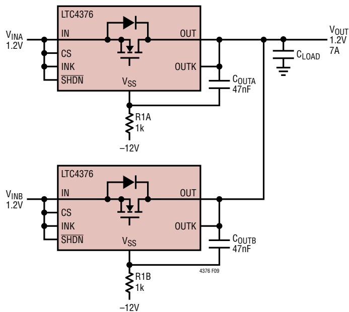
Figure 9. 1.2V Diode-OR
