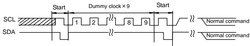
Figure 35-(b). The case of START + dummy clock x9 + START + command input
