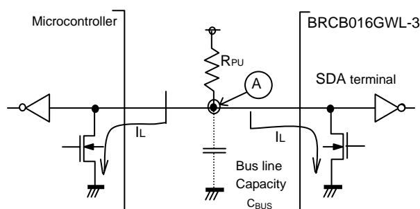
Figure 39. I/O circuit diagram
