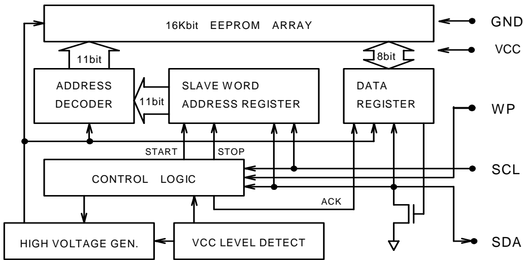
Figure 2. Block Diagram
