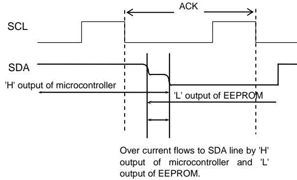
Figure 41. Input / Output Collision Timing
