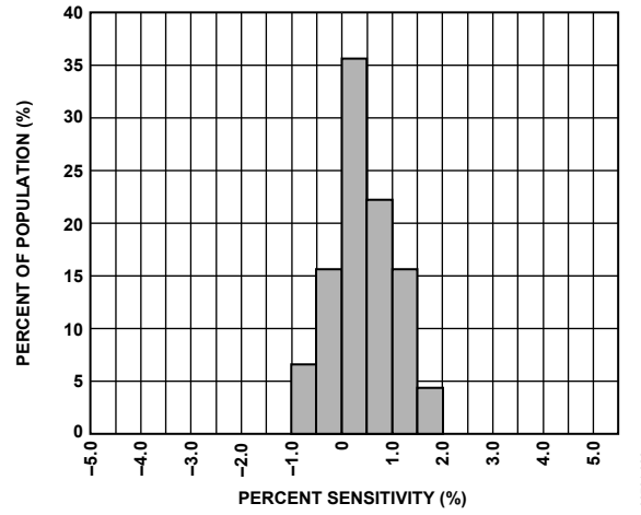
Figure 37. Z vs. Y Cross-Axis Sensitivity
